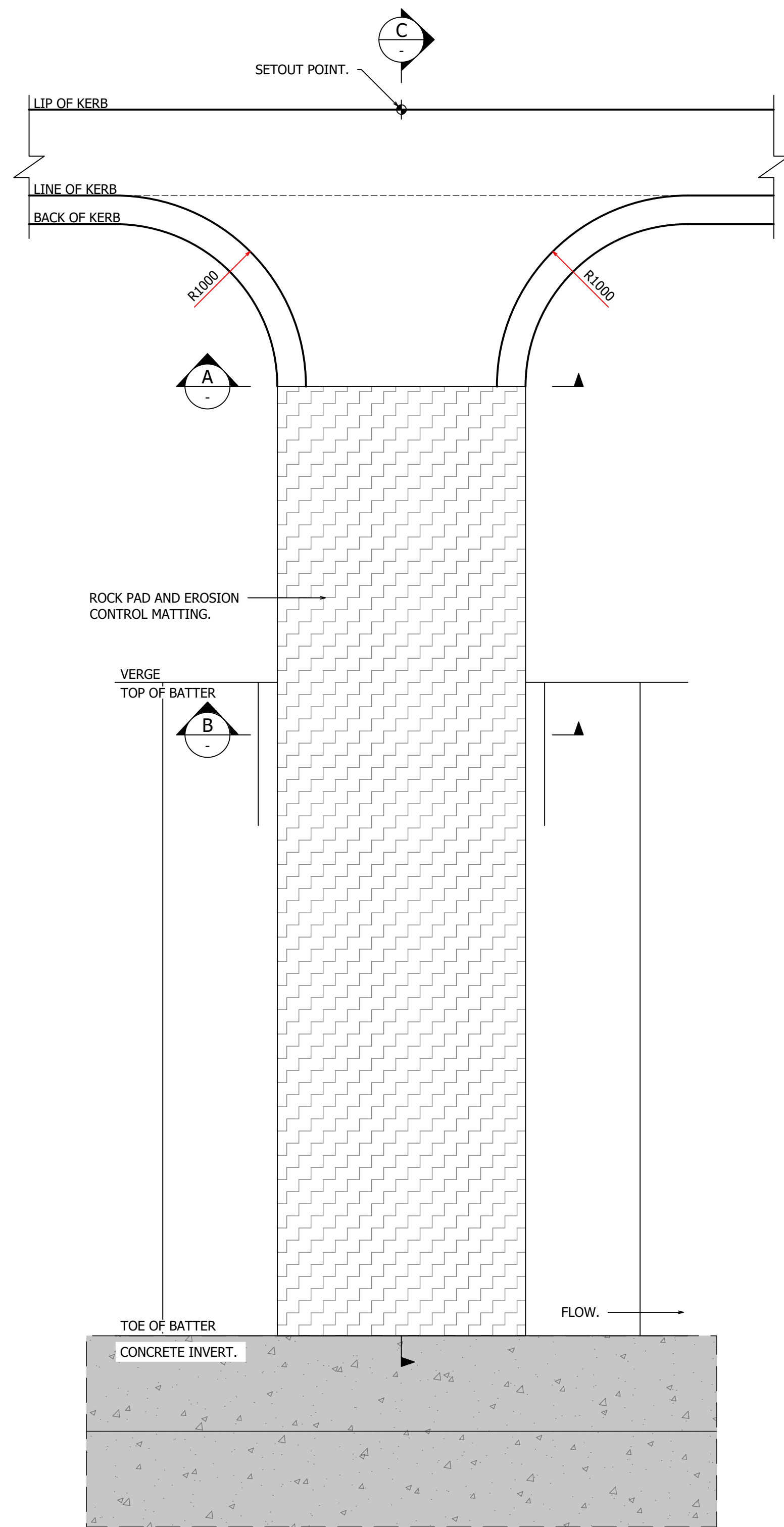
KERB OUTLET TYPICAL DETAIL PLAN N.T.S.
